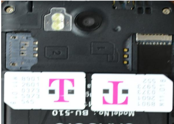
Full SIM Card Orientation
