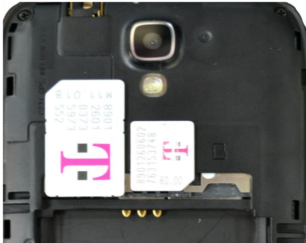
SIM Card Orientation
